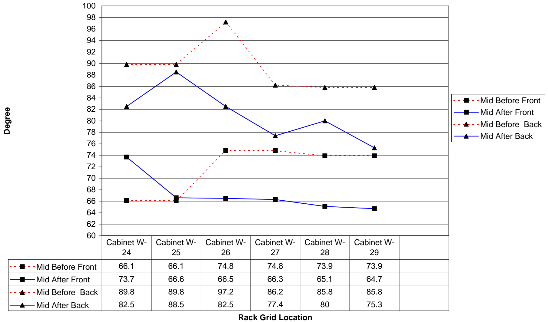
Readings Test-2 Temperature Graph - Middle of Rack
