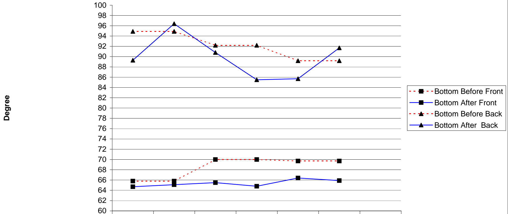
Readings Test-1 Temperature Graph - Bottom of Rack
