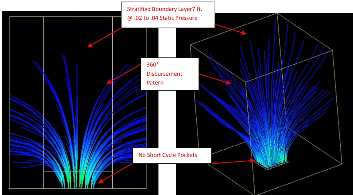
3 Legs of Passive Cooling: 1. Eliminate Short Cycle, 2. 360° Disbursement, 3. 7 ft. Stratification
