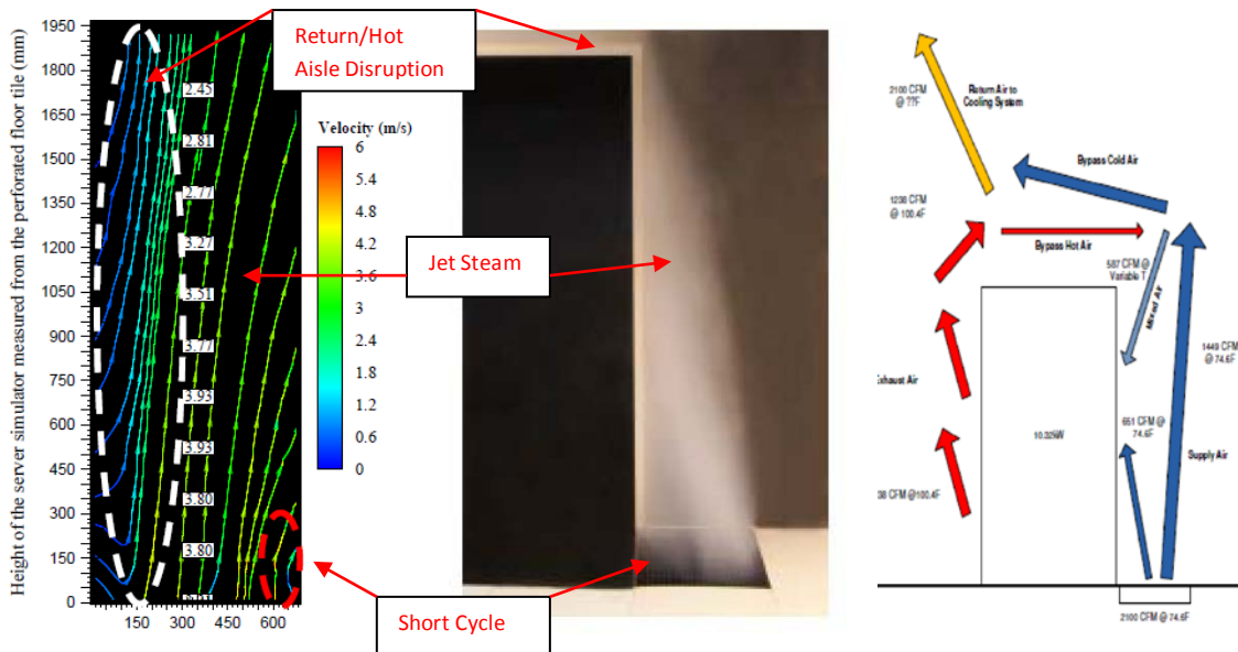
Jet Stream Contamination: 1. Short Cycle, 2. Lack Disbursement, 3. Return Air/Hot Aisle Disruption
